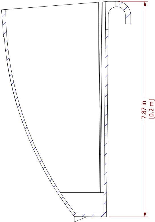
SECTION C-C SCALE 1 / 2
