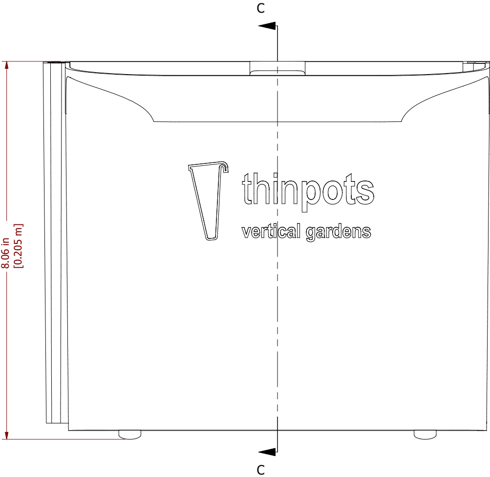
THINPOT DETAIL SCALE 1 / 2
