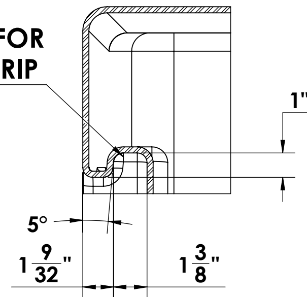
DETAIL C SCALE 1 : 4 (6 PLACES)
