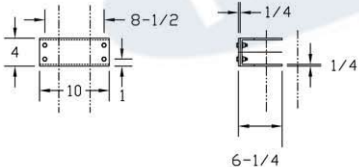
TYP. Bracket Detail
